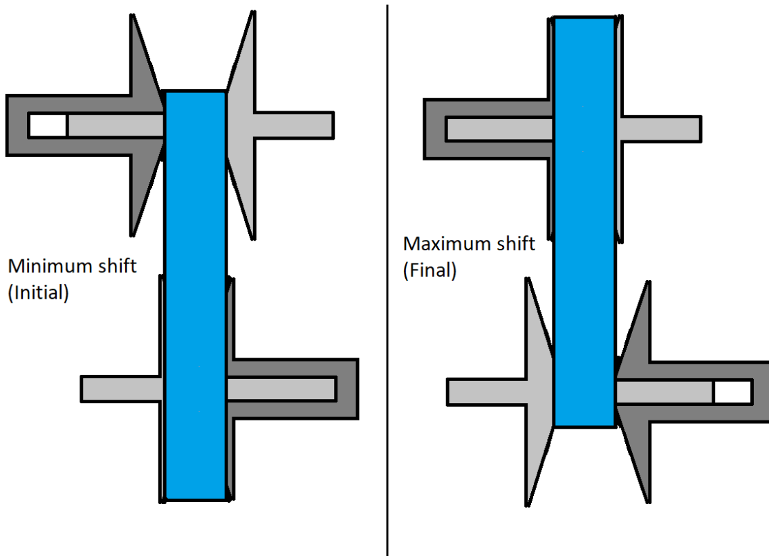
Figure 11: Conceptual illustration of variable pulley geometry. Changes in axial separation alter effective radii. Because belt length is constrained, an increase in primary effective radius corresponds to a decrease in secondary effective radius.
